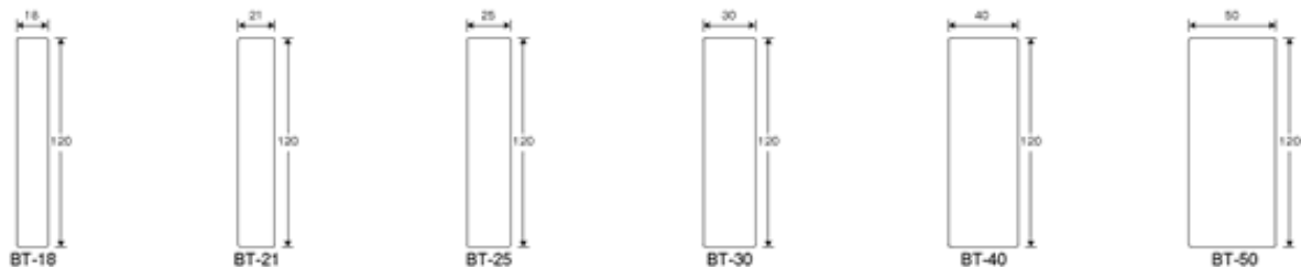
Test Tubes For Plant Culture reduced scale
