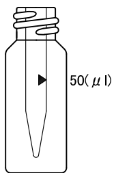
SPV-50 (11.75 × 32)
