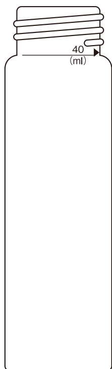
EPA-40 (27.5 x 95)
