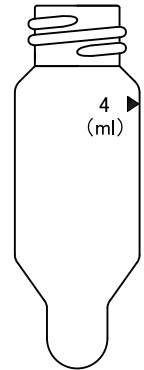
MV-2 (16.5 × 48)
